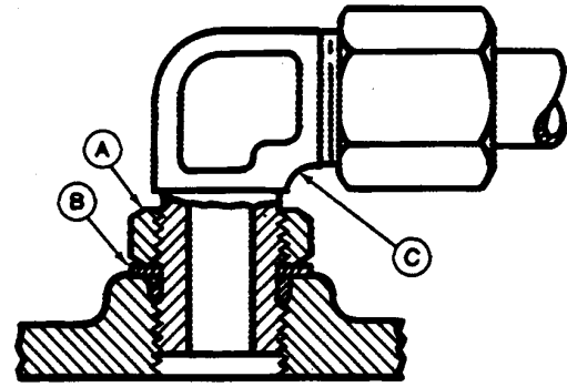
Angle Fitting
